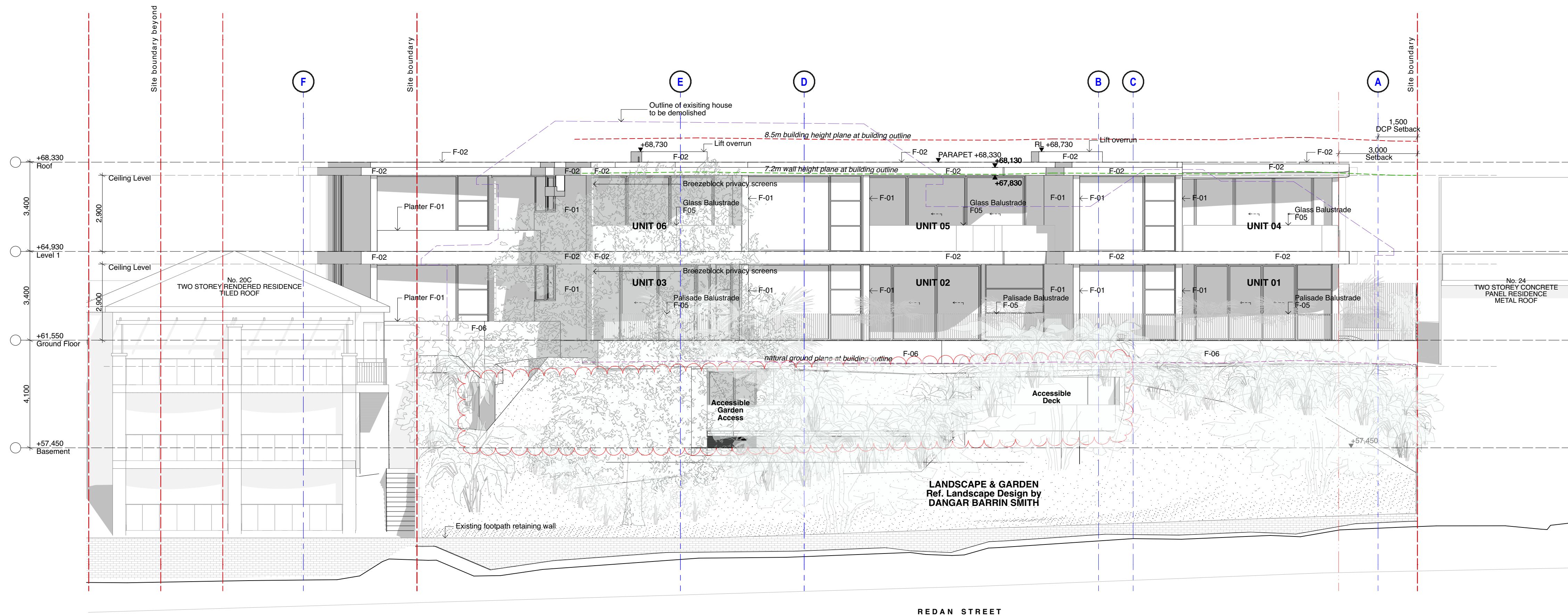
EAST ELEVATION
